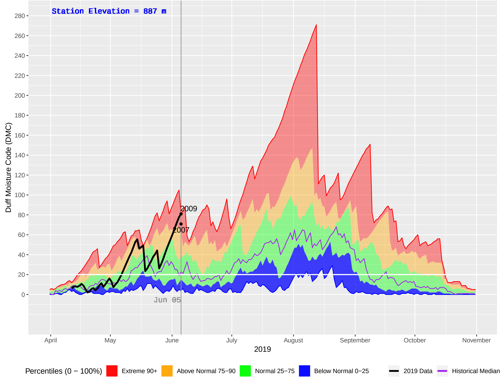
CRAWFORD (873) : Historical (2004–2018), Current (2019) Daily Duff Moisture Code (DMC)
