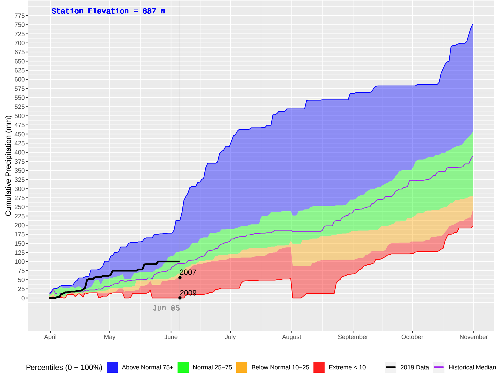
CRAWFORD (873) : Historical (2004–2018), Current (2019) Daily Cumulative Precipitation
