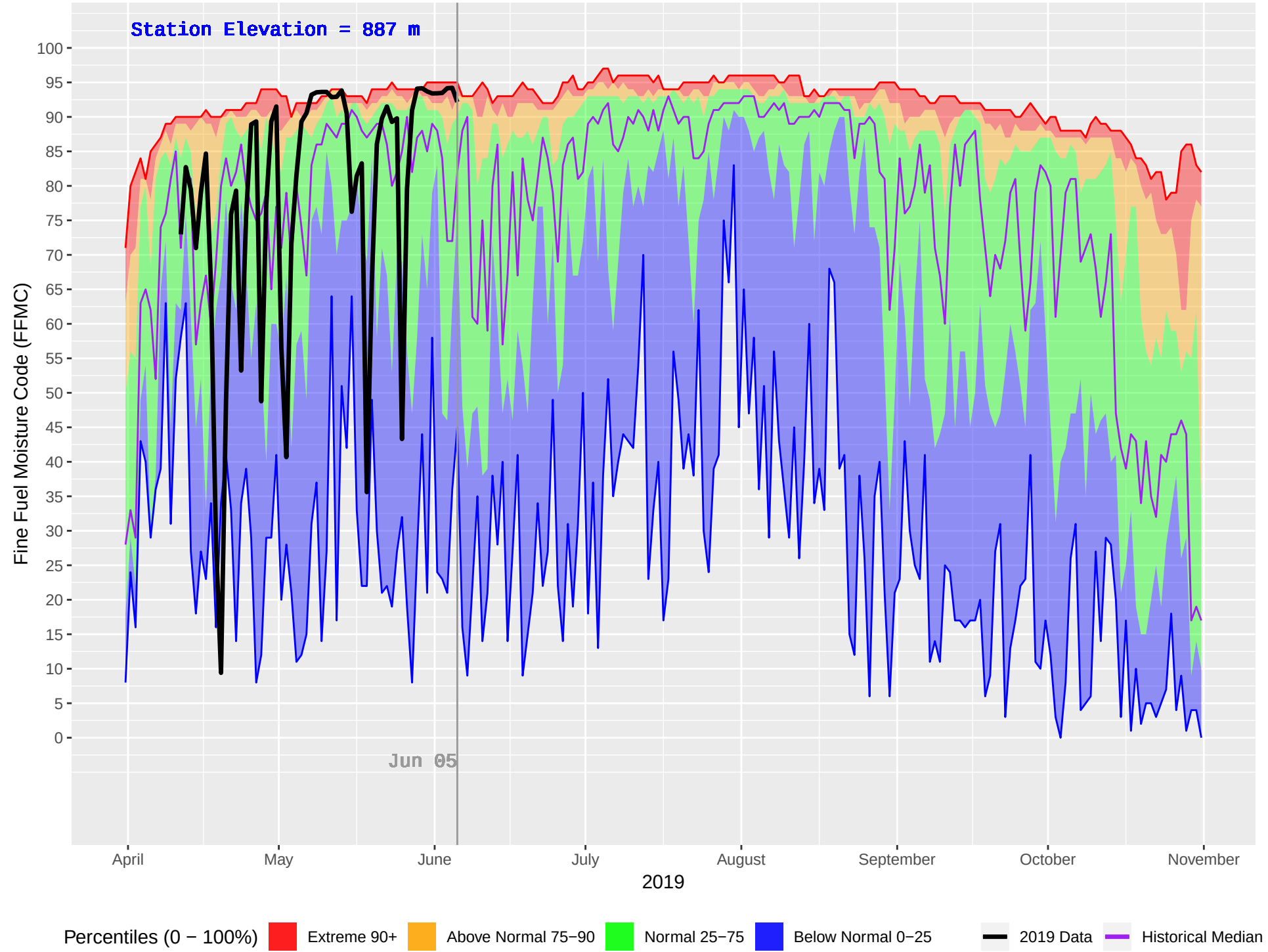
CRAWFORD (873) : Historical (2004–2018) and Current (2019) Daily Fine Fuel Moisture Code (FFMC)
