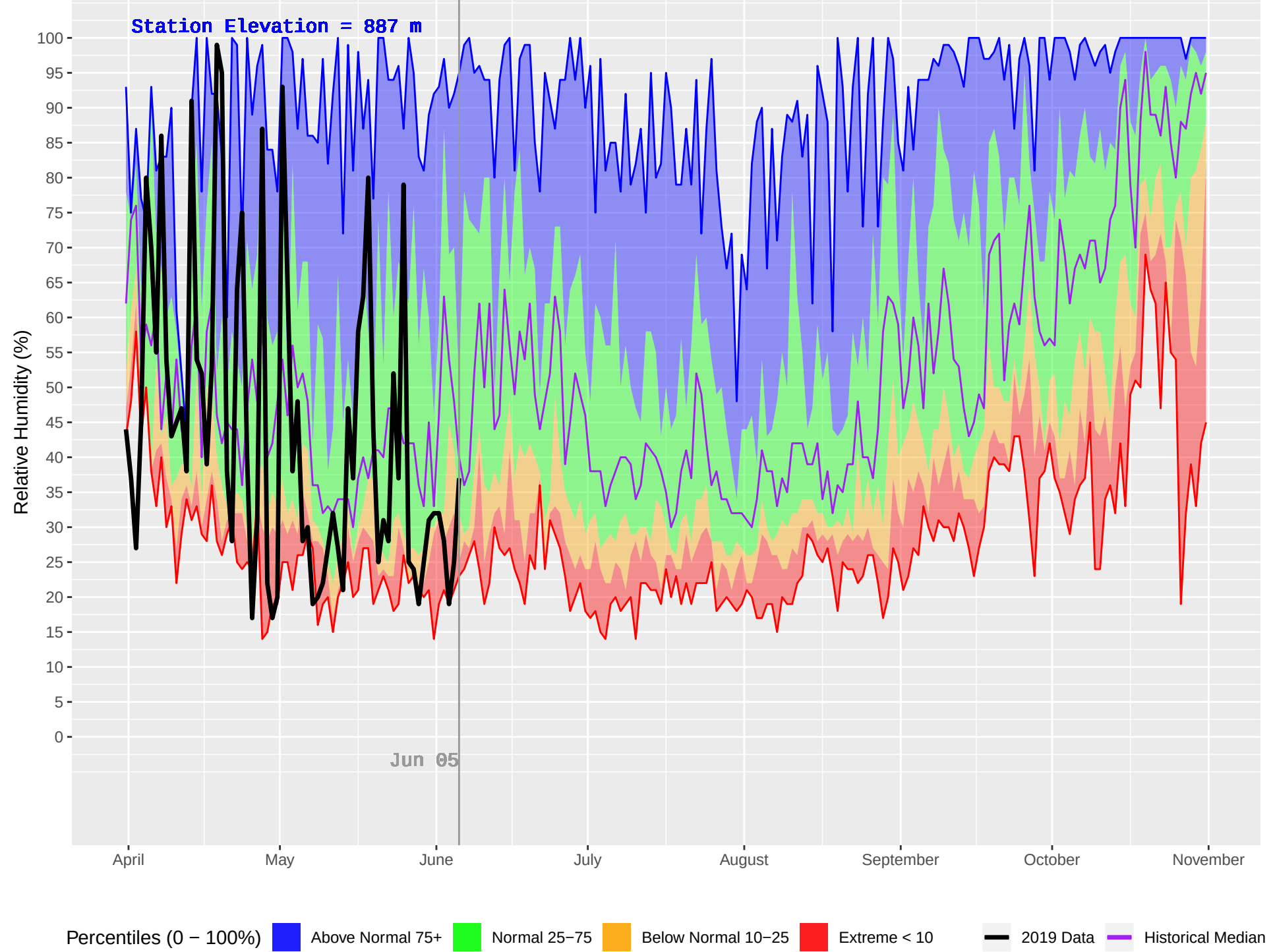
CRAWFORD (873) : Historical (2004–2018) and Current (2019) Daily Relative Humidity
